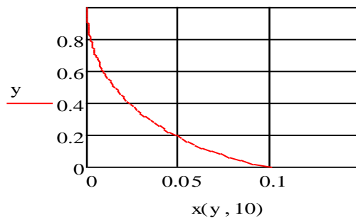
Figure 4. Pursuit curve at \alpha = 10 .
