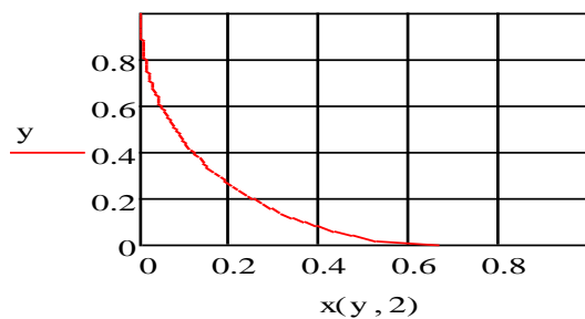
Figure 2. Pursuit curve at \alpha = 2 .
