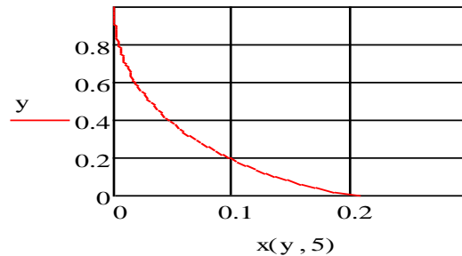
Figure 3. Pursuit curve at \alpha = 5 .
